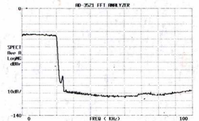
● -20dB, White noise, Spectrum (Direct Out)
