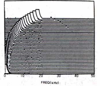
● -20dB, White noise, Spectrum (Direct Out)
