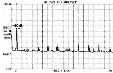
● -80dB, 997Hz, Spectrum (Direct Out)
