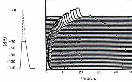
● -80dB, 997Hz, Spectrum (Direct Out)
